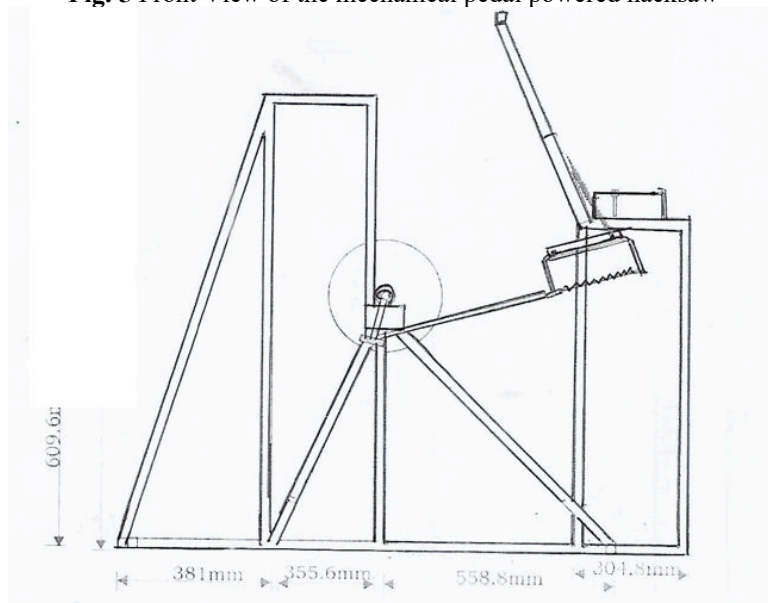
Fig. 6 Side View of the mechanical pedal powered hacksaw
