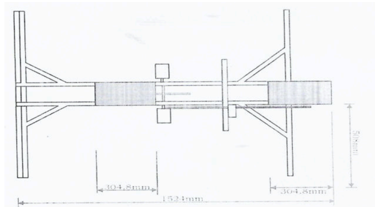
Fig. 7 Plan of the mechanical pedal powered hacksaw
