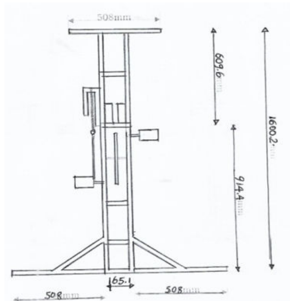
Fig. 5 Front View of the mechanical pedal powered hacksaw
