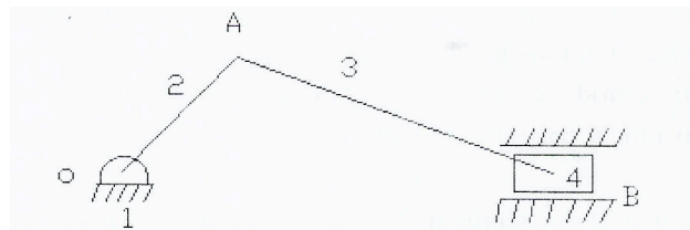
Fig. 1 Single slider crank mechanism
