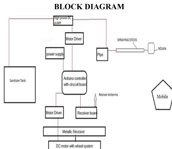
Fig. 1 Block Diagram
