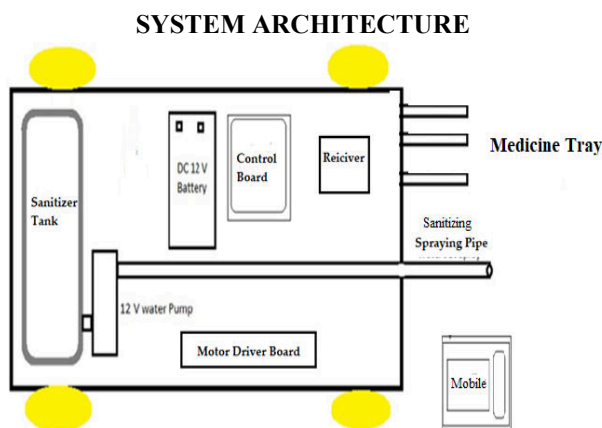
Fig. 2 System Architecture
