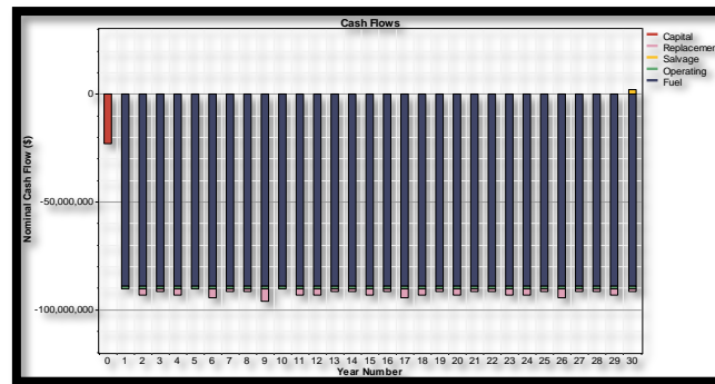
Fig. 8 Cash flow for Diesel Costing 0.9$/l
