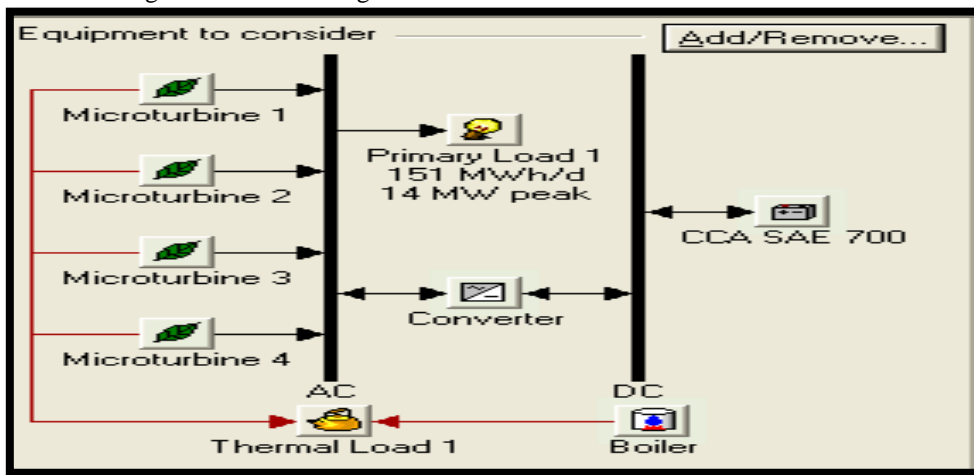
Fig. 4 Case 1 HOMER schematic model
