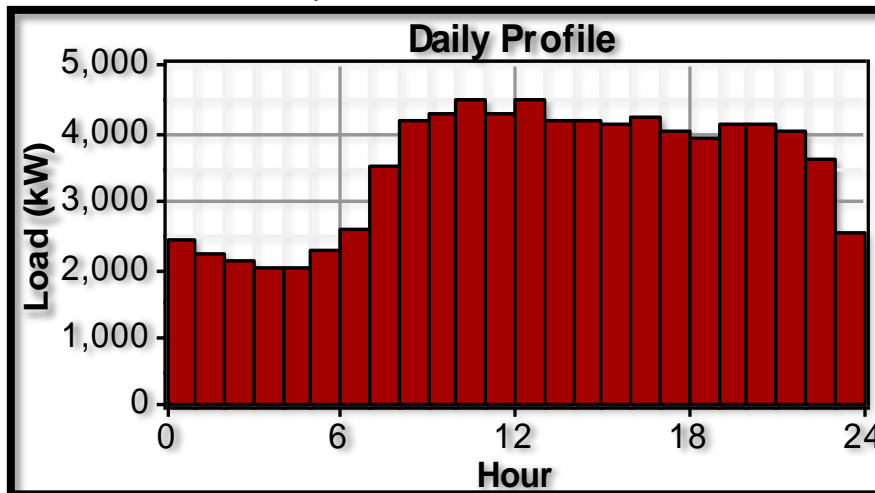
Fig. Error! No text of specified style in document. Thermal load daily profile for Cape Town households in winter [9]
