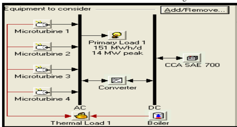
Fig. 7 Case 2 Homer Schematic
