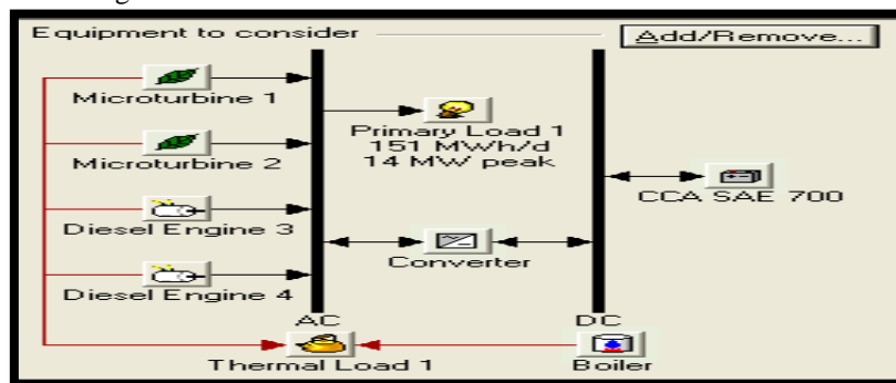
Fig. 1 Case 3 HOMER Model Schematics
