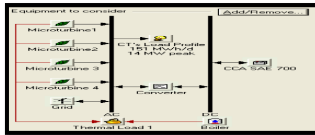
Fig. 4 Case 4 HOMER model schematic
