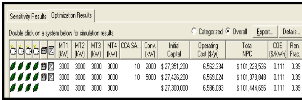
Fig. 5 Optimization results for case 1 System
