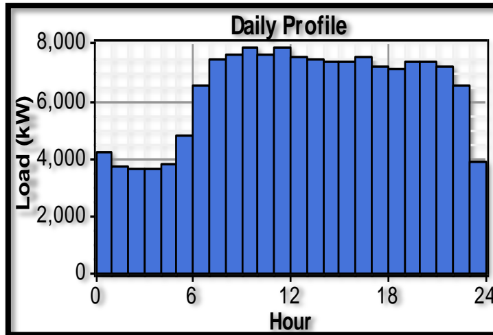
Fig. 2 Electric daily profile data for Cape Town households in winter [9]
