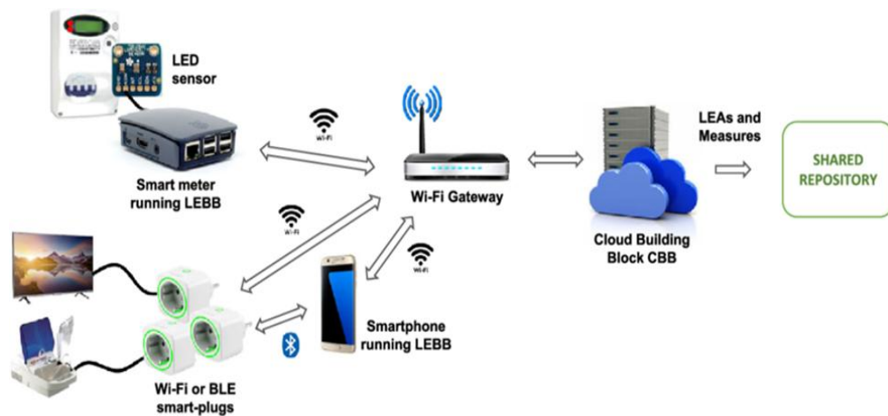
Figure 1: IT Infrastructure [16]
